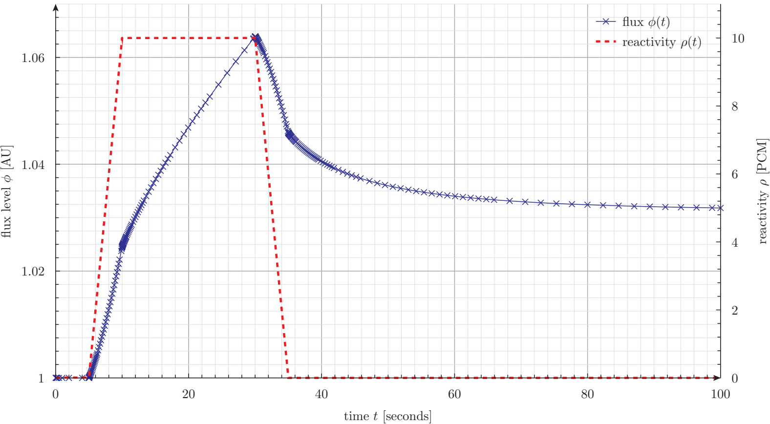
Point reactor equations with \rho(t) given as scattered data
